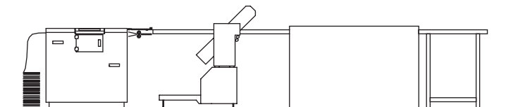
CUTTER TC 7022 T TC 1007 T FOLDER INSERTER CONVEYOR TC 0250
