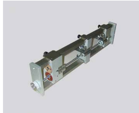
SIDE TRIMMING & CENTRAL KNIFE CARTRIDGE TC 1003
